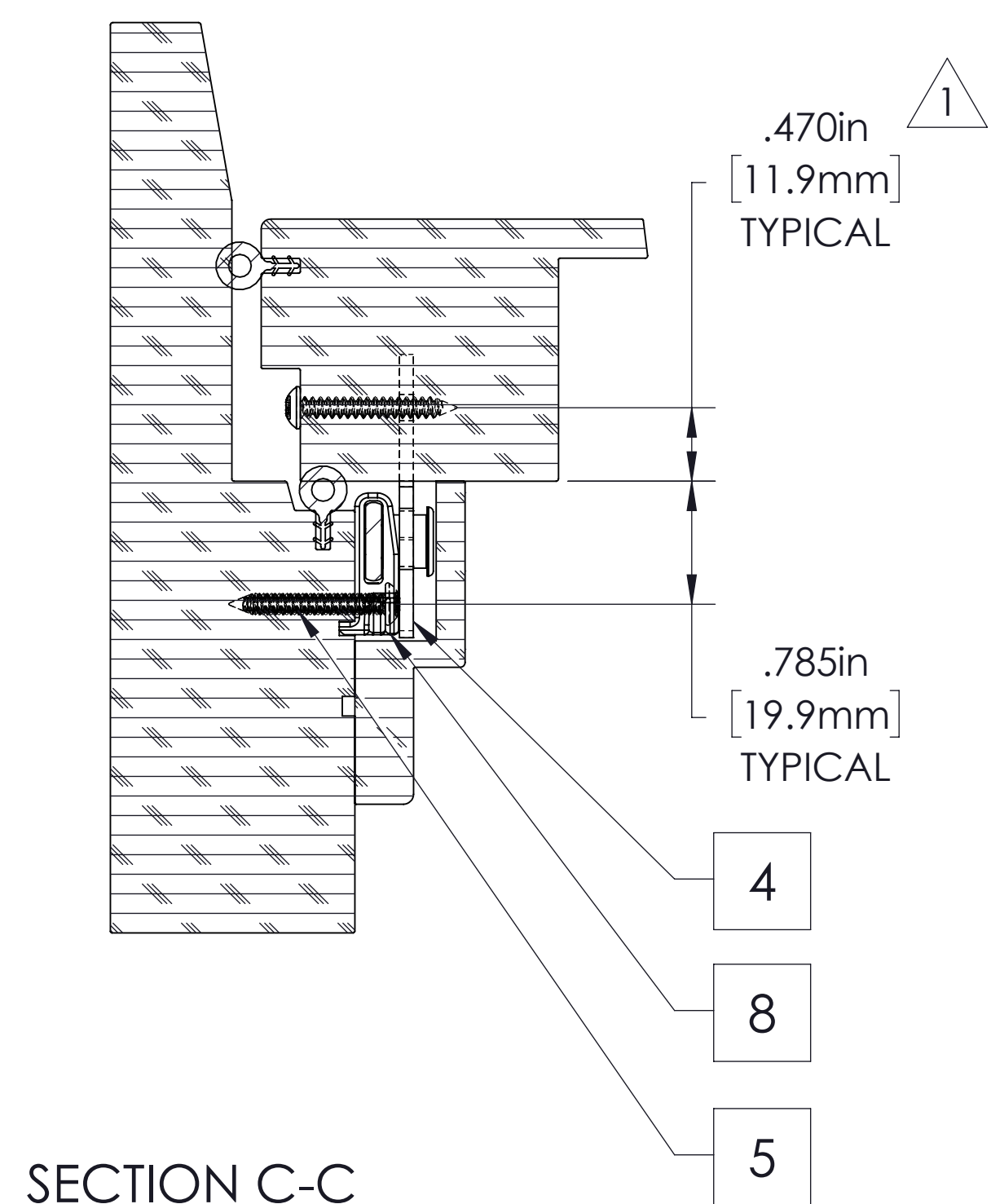
SECTION C-C SCALE 1 : 1
